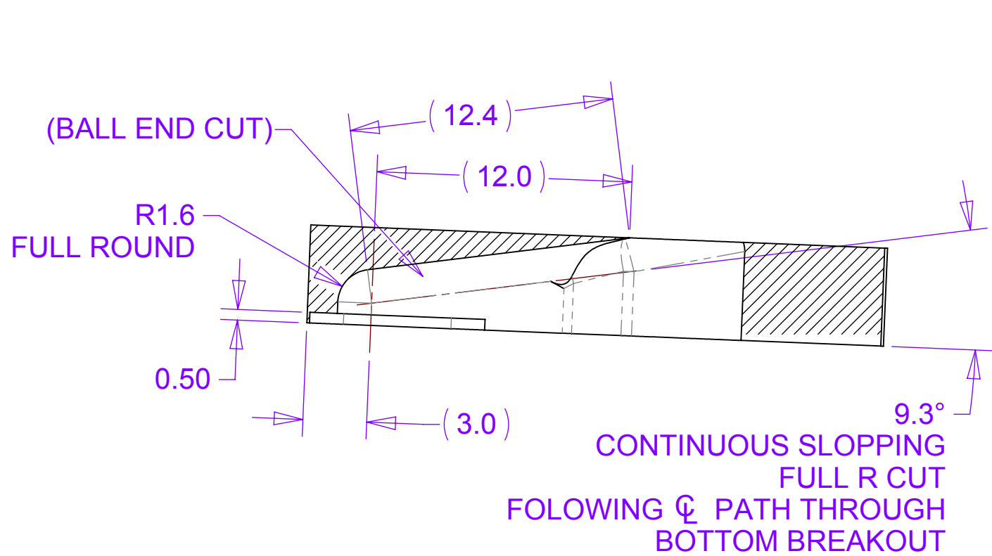
SECTION E-E
