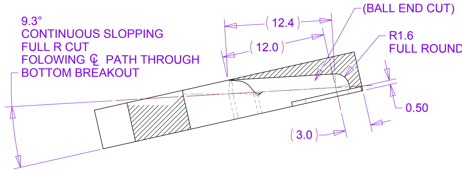
SECTION F-F
