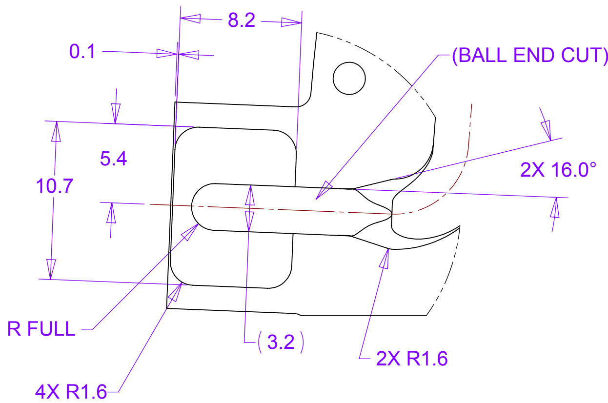
DETAIL K VIEW TYP 2X
