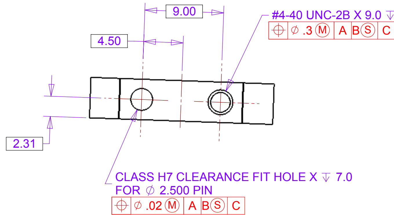
SECTION B-B
