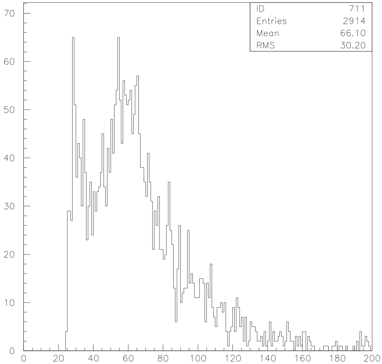
charge deposited histogram. 1 and 2 strip clusters.
